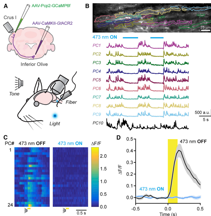
Figure 3. Dendrite-wide \text{Ca}^{2+} Signals in PCs Are Completely Mediated by CFs
