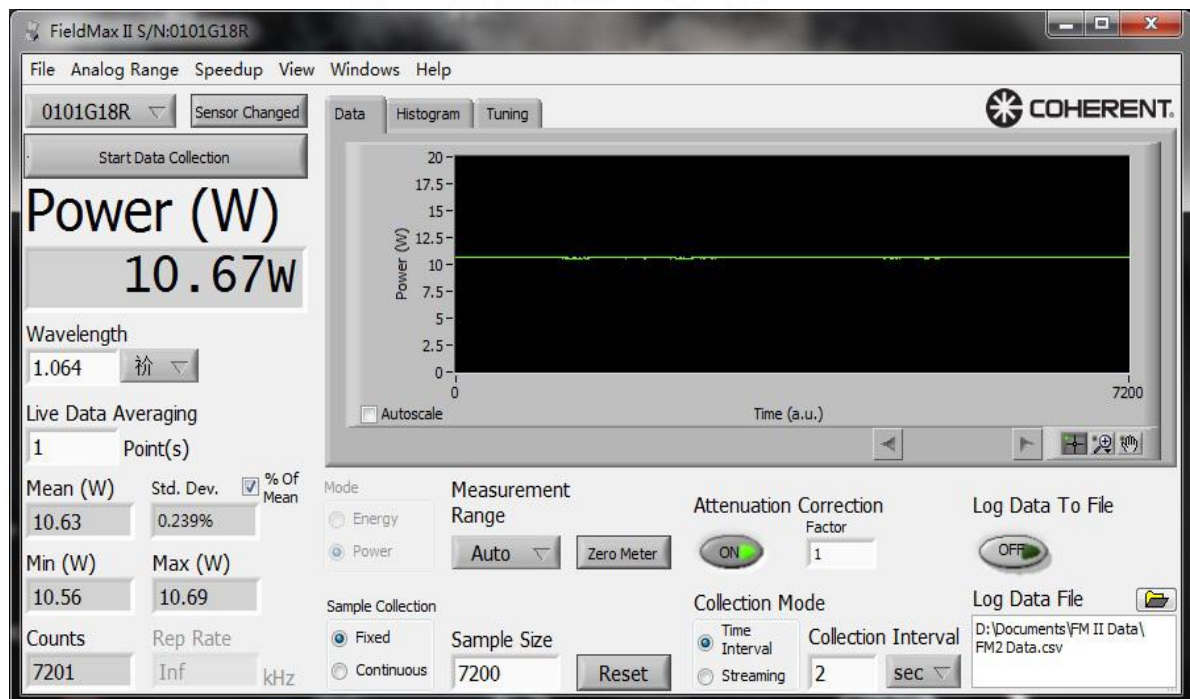
Graph 2: Output power and Stability testing
